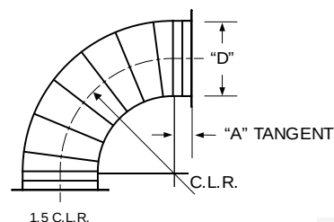
PART NO. 3211
