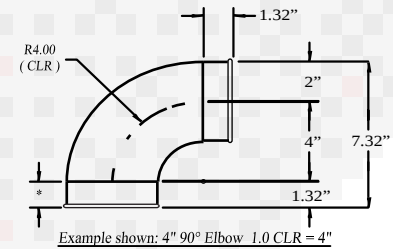
PART NO. 3210
