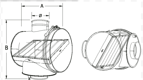
PART NO. 3192
