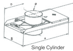
Single Cylinder
