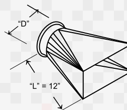
PART NO. 3232
