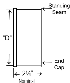
Part No. 3151
