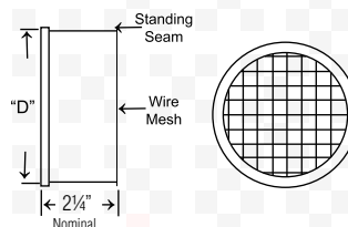
Part No. 3152
