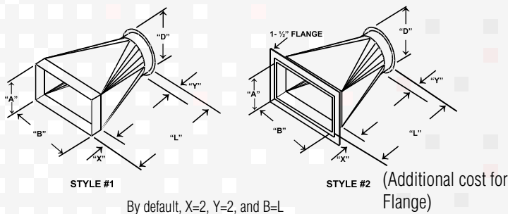
PART NO. 3225
